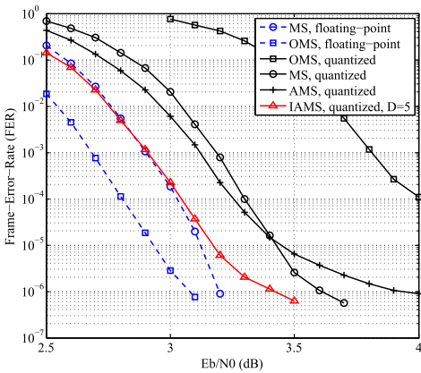
Fig. 7. Simulation results on the R = 2/3 , Z = 104 , N = 3432 BG1 code when I_{t_{max}} = 100 .
