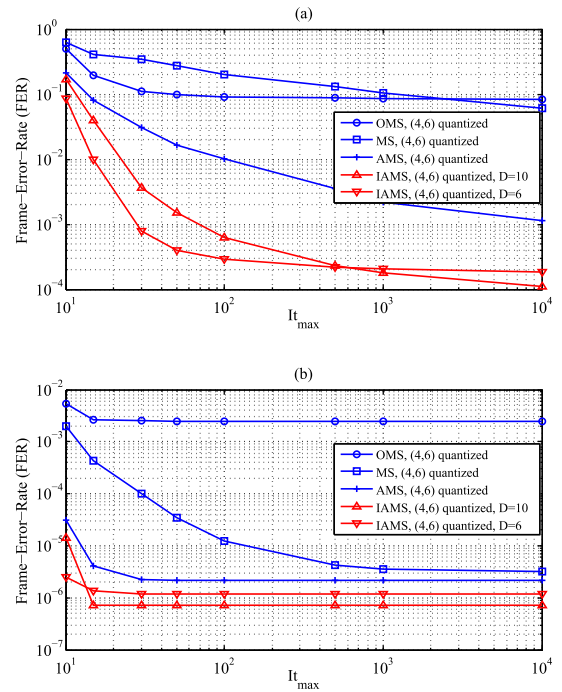
Fig. 8. FER performance under different iteration limits at (a): E_b/N_0 = 2.0 dB, (b): E_b/N_0 = 2.6 dB.
