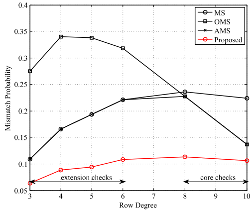
Fig. 2. The mismatch probabilities of different CN-update functions under the row degree region for BG2 codes.
