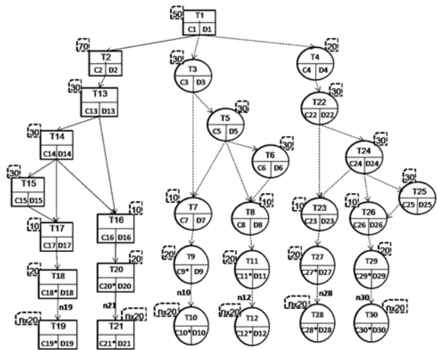
Figure 3. Our proposed model for the robotic vision application
