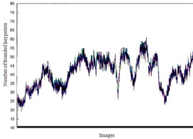
Figure 5. Number of detected keypoints in image sequence
