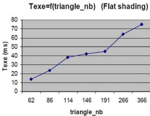
Figure 2. Texte/triangle_nb variation for flat shading
